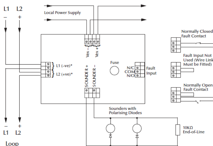
Figure 1 Sounder Control Unit with Isolator Wiring Diagram
