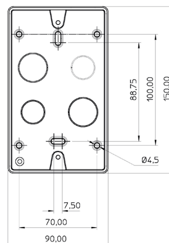
Figure 2 Sounder Control Unit with Isolator
