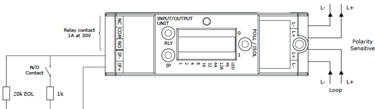
Figure 3: Intelligent DIN-Rail Input/Output Unit normally open monitoring mode connectivity diagram (compatible with CoreProtocol only)
