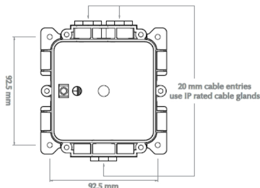
Figure 1: Waterproof Addressable Manual Call Point Backbox
