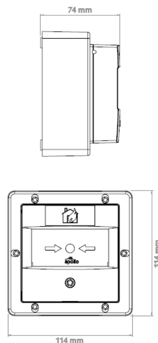
Figure 2: Waterproof Addressable Manual Call Point dimensional drawing
