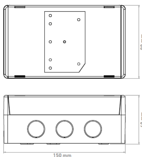
Figure 1: Intelligent Mains Switching Input/Output Unit dimensional drawing
