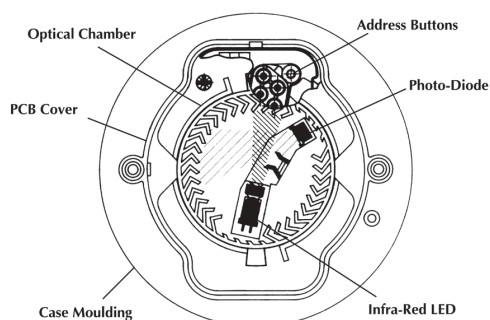
Top Section - XP95 Optical Smoke Detector
