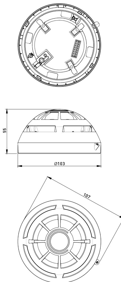
Figure 1 – Soteria Tri-Sensor Detector (Dual Optical/Heat/CO) dimensional drawing
